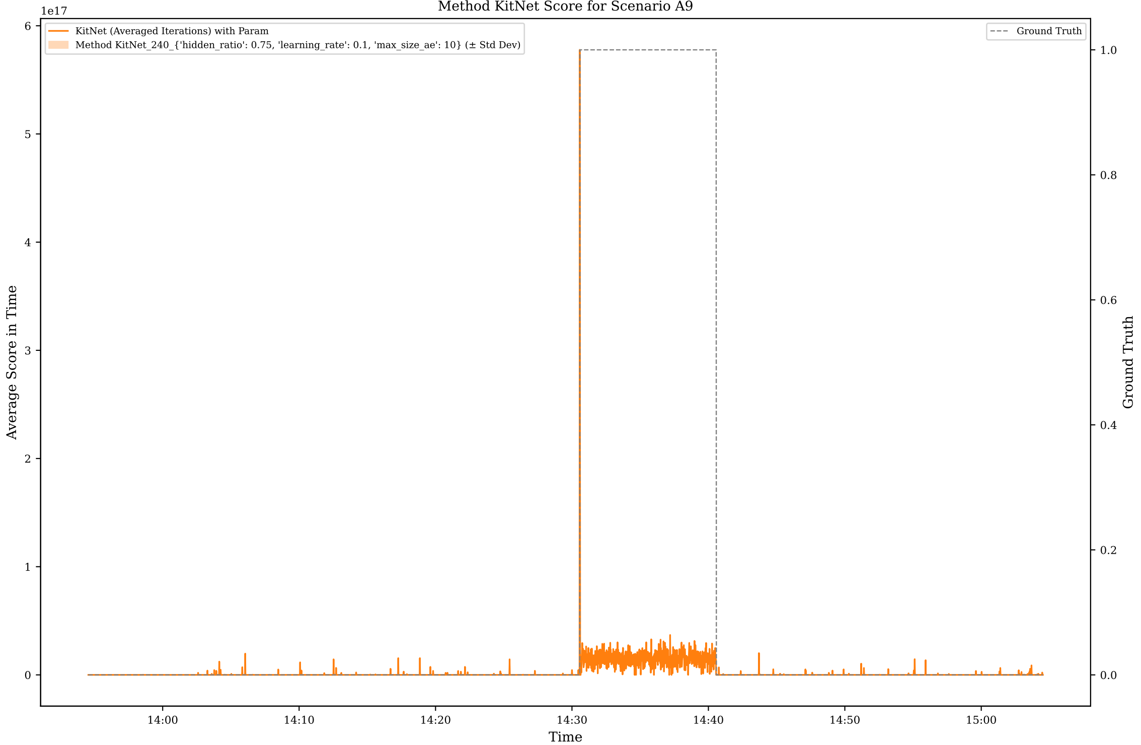
Method KitNet Score for Scenario A9
